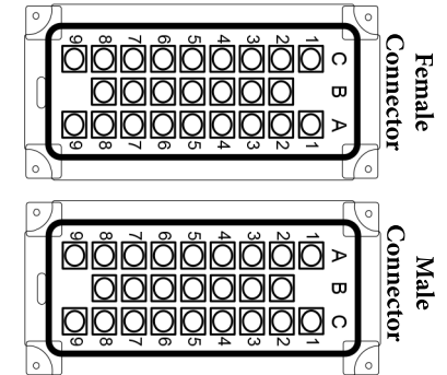
12-ZONE / 25-PIN STANDARD HEATER
