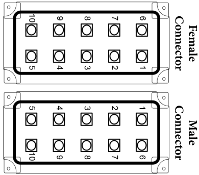
5-ZONE / 10-PIN STANDARD HEATER
