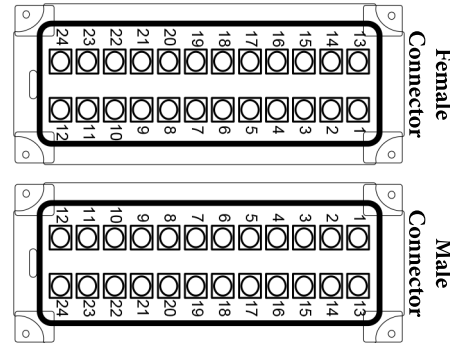
12-ZONE / 24-PIN STANDARD HEATER
